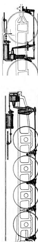
Fig. 2559. Arrangement of Equalized Driver Brake on Four Pairs of Wheels.
